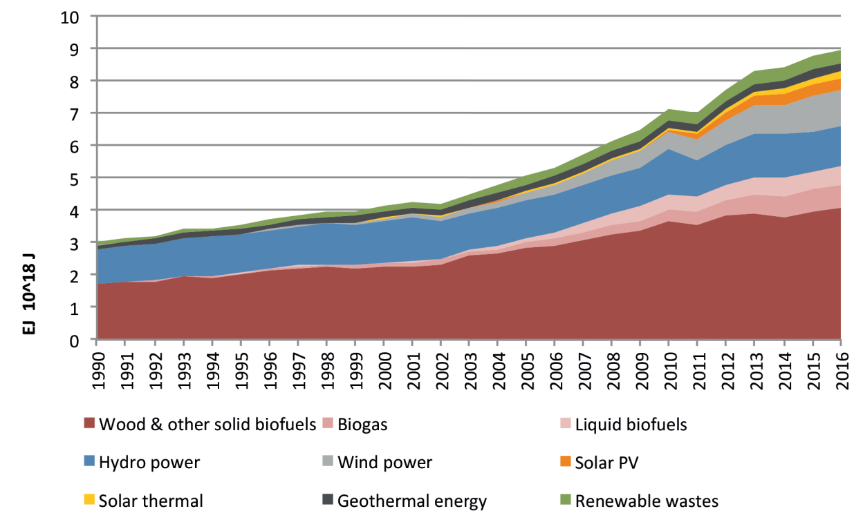
Figure 10: Shares of Renewable Energies in primary energy production with time.
