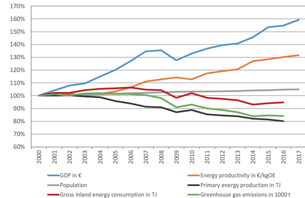
Figure 14: Temporal development of GDP, energy productivity (GDP per gross inland energy consumption), population, primary energy production, gross inland consumption and greenhouse gas emission. (Year 2000=100%). Data taken from https://ec.europa.eu/eurostat/web/energy/data/main-tables 16
