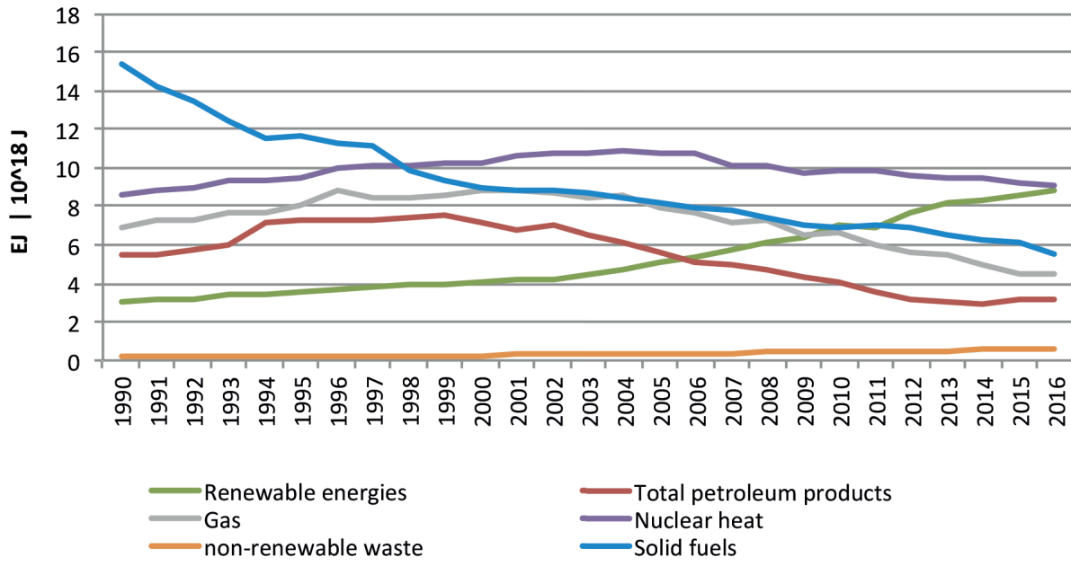
Figure 7: Primary energy production in EJ (10 18 J) of the EU-28 from 1990 until 2016.
