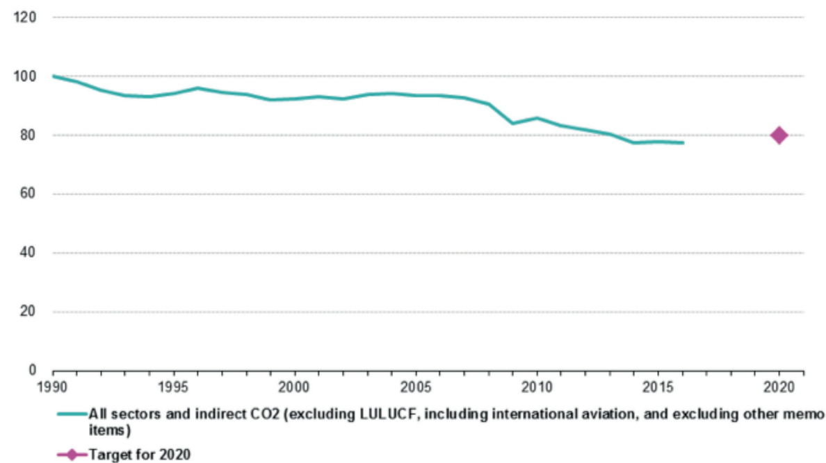
Greenhouse gas emissions, EU-28, 1990-2016 (index 1990 = 100)
