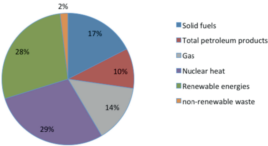
Primary energy production by resource EU-28 in 2016
